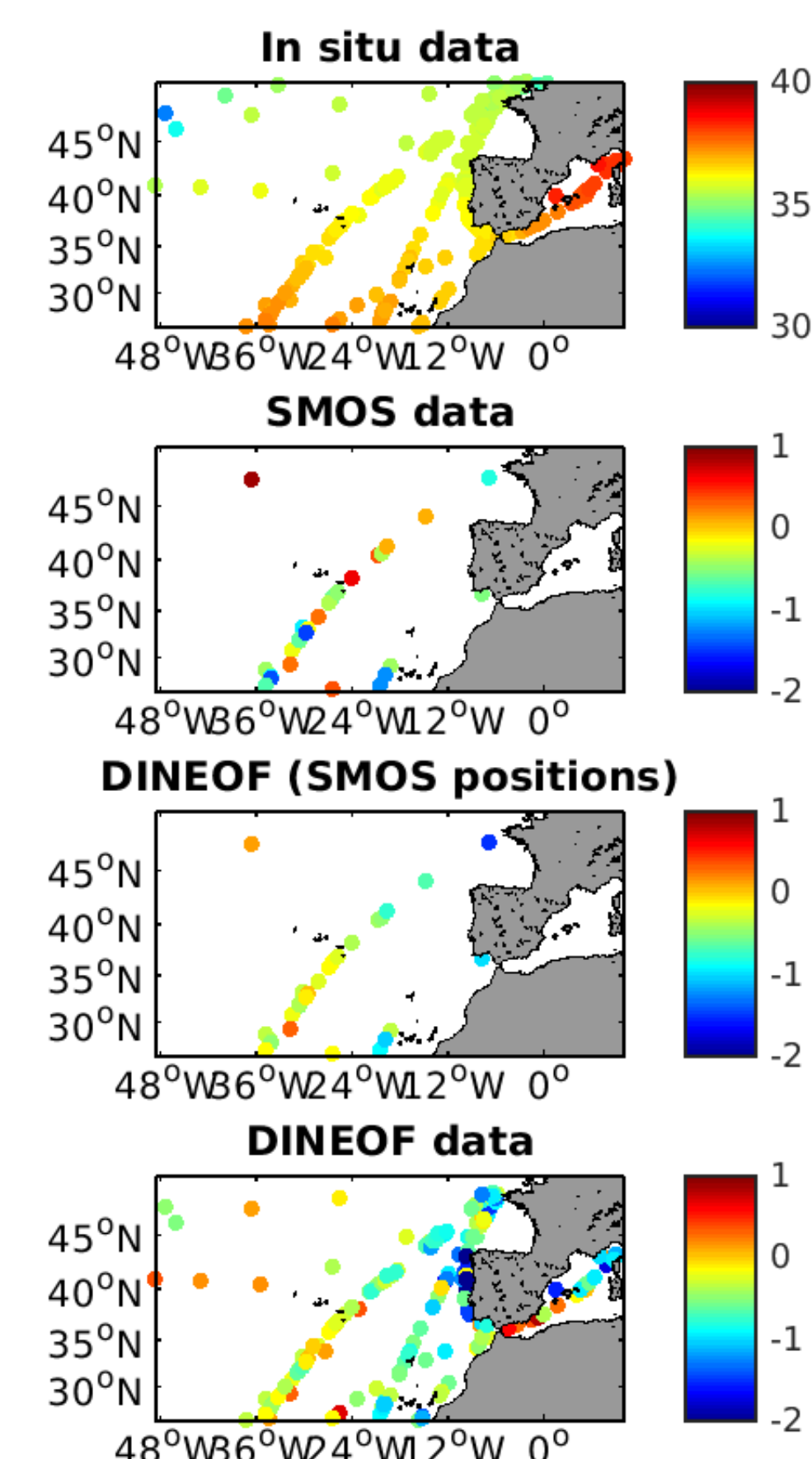
Figure 3: First panel: TSG data, averaged daily. Second panel: original SMOS SSS data anomalies with respect to the TSG data. Third panel: DINEOF reconstruction of SSS data (anomalies with respect to the TSG data) at the initially present SMOS positions. Fourth panel: DINEOF reconstruction of SSS data anomalies with respect to the TSG data at all positions.
